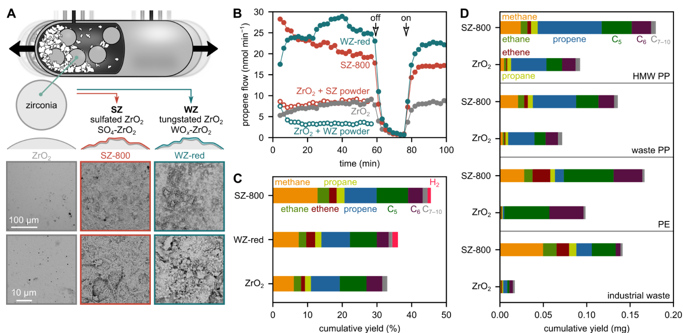
Figure 1. Mechano-catalytic conversion of plastic (waste) to C 1-10 hydrocarbons. (A) Milling container, surface activation strategy, and SEM images of grinding spheres. (B) Propene flow during milling of 2 g model PP with sulfated (SZ-800), tungstated (WZ-red), and untreated (ZrO 2 ) spheres at 30 Hz, compared to milling with untreated spheres and 0.1 g SZ and 0.2 g WZ powder catalysts. The shaking was turned off/on at the indicated points. (C) Cumulative yields during milling of 20 mg model PP for 1 h at 35 Hz with sulfated (SZ-800), tungstated (WZ-red), and untreated (ZrO 2 ) spheres. (D) Cumulative yields during milling of HMW PP (2 g, 30 Hz), waste PP (2 g, 30 Hz), PE (2 g, 35 Hz) and industrial waste (1 g, 30 Hz) for 1 h with sulfated (SZ-800) and untreated (ZrO 2 ) spheres.
